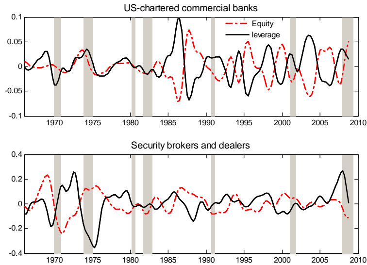
Figure 2: Cyclical components of intermediary leverage and equity
