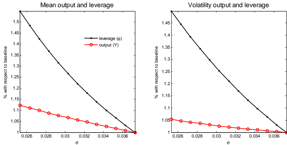
Figure 7: The effect of changes in steady-state cross-sectional volatility
