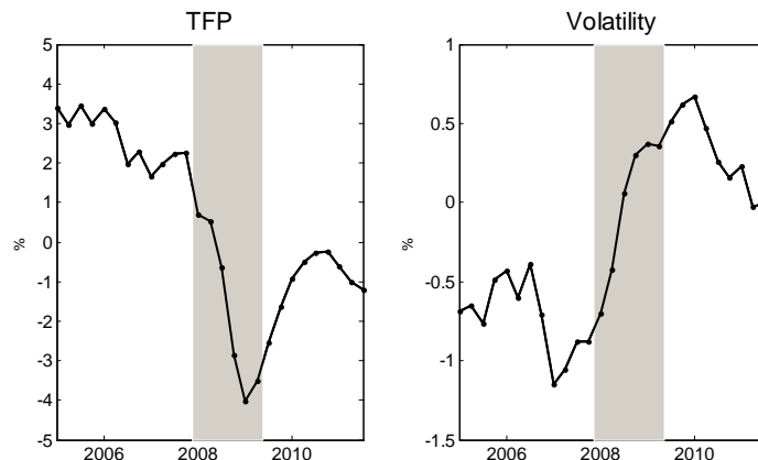
Figure 5: Smoothed series for the exogenous processes
