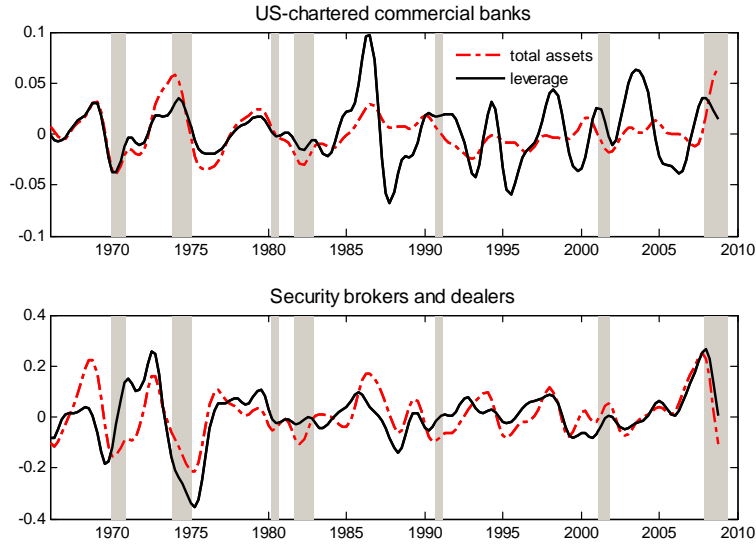
Figure 1: Cyclical components of intermediary leverage and total assets
