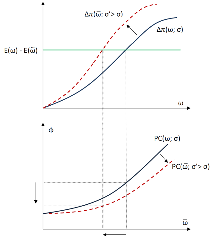
Figure 3: The volatility-leverage channel
